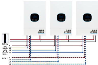
3 Phases parallel connection
