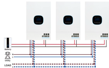
Add Power Parallel Connection
